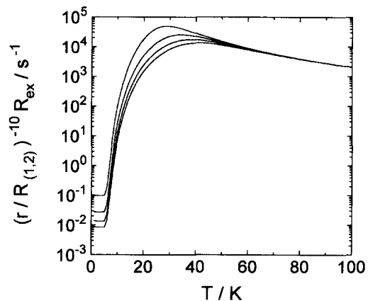
Fig. 2. (R_{(1,2)}^{(0)}/r)^{10} R_{\text{ex}}/s versus temperature according to Eq. (8) for V_3^{(1)} = 15B and V_3^{(2)} = 15.5, 16, 16.5, 17B , from top to bottom. The remaining parameters are the same as in Fig. 1.
