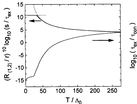
Fig. 1. Upper curve: (R_{(1,2)}^{(0)}/r)^{10} \log(s/\tau_{\text{ex}}) , lower curve: \log(\tau_{\text{ex}}/\tau_{\text{con}}) for R_{(1,2)}^{(0)} = 5r versus temperature in units of the tunnelling energy \Delta corresponding to V_3^{(1)} = V_3^{(2)} = 20B . Debye phonons have been assumed with \omega_D = 18B , g_k^c = g_k^s and g := g_k^{c/s}/\sqrt{V_3^{(\alpha)}\omega_k} = 0.1 . At temperatures T \gtrsim 95\Delta the conversion becomes more rapid than the exchange.
